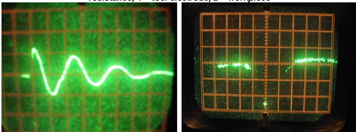
Fig. 2. Overview of the pulse current for the capacity value C = 1/12 \mu\text{F} , the ballast resistance R = 8.2 \text{ M}\Omega : a) time division size 1 \mu\text{s}/\text{div} , voltage division size 100 \text{ V}/\text{div} ; b) time division size 0.1 \mu\text{s}/\text{div} , voltage division size 100 \text{ V}/\text{div}
