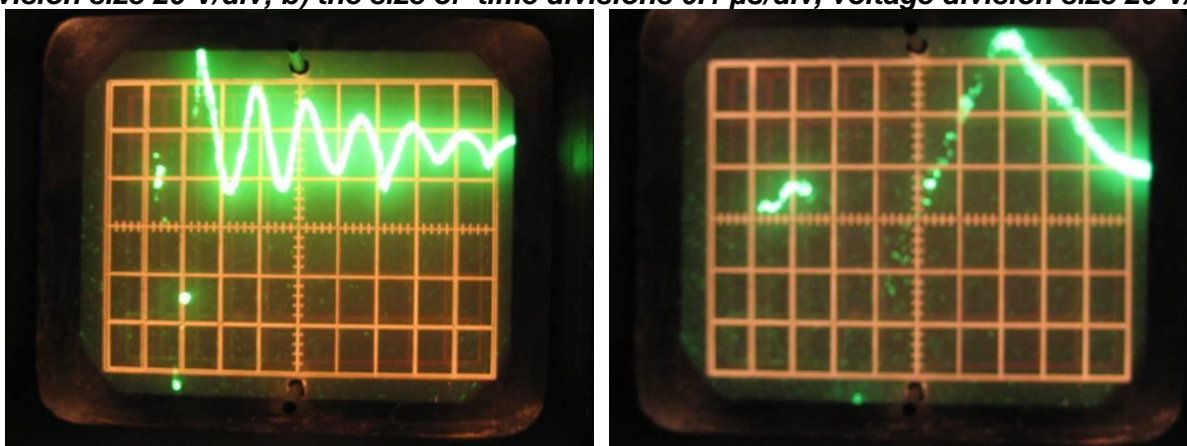
Fig. 4. Overview of the pulse current for the capacity value C=17.5 \text{ nF} , the ballast resistance R=8.2 \text{ M}\Omega : a) the size of time divisions 1 \text{ }\mu\text{s/div} , voltage division size 20 \text{ V/div} ; b) the size of time divisions 0.1 \text{ }\mu\text{s/div} , voltage division size 20 \text{ V/div}
