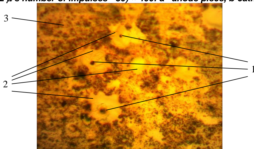
Fig. 7. A portion of the brass surface L63 machined with electric discharges in impulse (the energy released in the interstice W = 8J , the interstice size S = 5mm gap size, impulse duration \tau_{imp}=0,2 \mu s the piece- cathode), \times 400 : 1 - meniscuses formed as a result of the "warm" electrode spots; 2 - the zone of thermal influence formed as a result of the "cold" electrode spots; 3 - the raw zone
