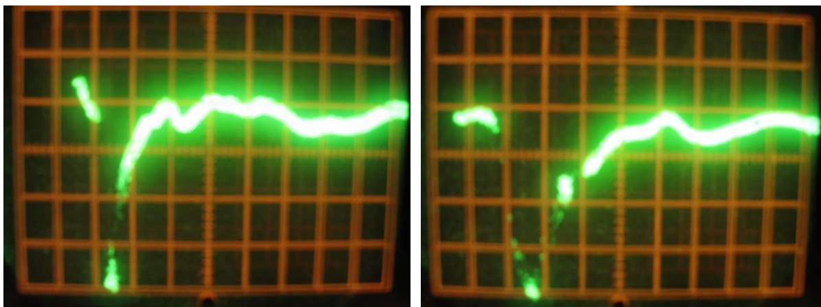
Fig. 3. Overview of the pulse current the for capacity value C = 5 \text{ nF} , the ballast resistance R = 8.2 \text{ M}\Omega : a) the size of time divisions 0.2 \text{ }\mu\text{s/div} , voltage division size 20 \text{ V/div} ; b) the size of time divisions 0.1 \text{ }\mu\text{s/div} , voltage division size 20 \text{ V/div}
