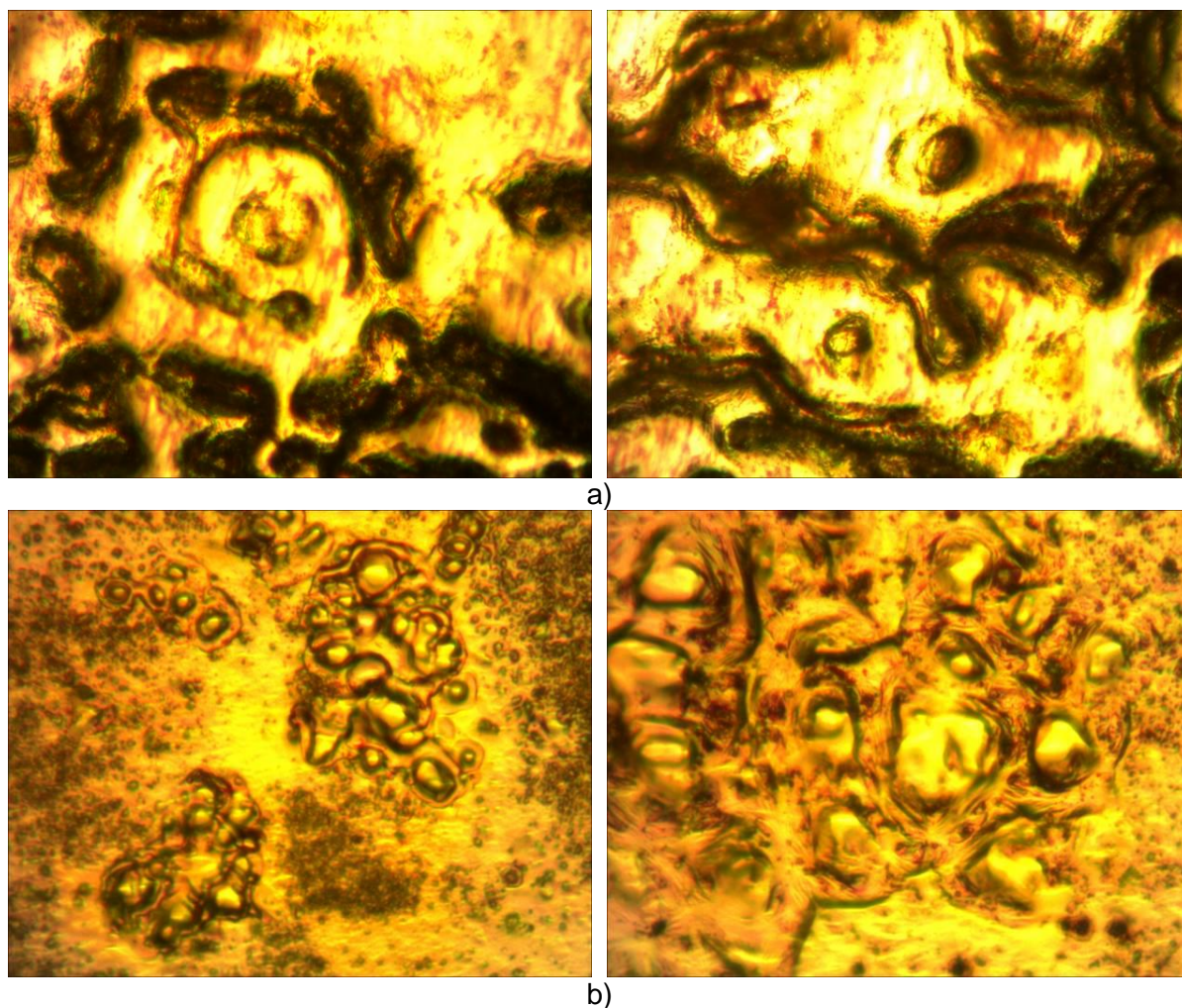
Fig. 6. Overview of L63 brass surface processed with electric discharges in impulse (energy released in the interstice W = 8J , the size of the interstice S = 5mm , the impulse duration \tau_{imp} = 0.2 \mu s number of impulses - 30) \times 400 : a – anode piece, b-cathode piece
