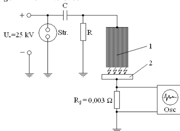
Fig. 1. The main scheme of the experimental installation and of measuring the pulse discharge parameters: Str. – perforator; Osc – oscilloscope with memory; R_s – shunt resistance; 1 – tool electrode, 2 – workpiece
